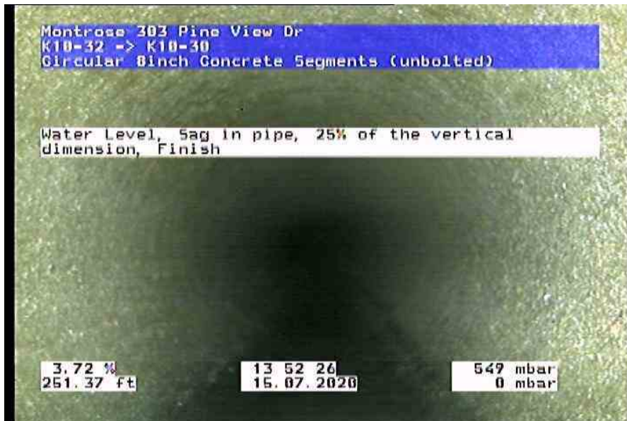
2228_af8e0d99-17f3-452d-94d7-e15e95241195_20200715_135750_899.jpg, 00:22:15, 251.37ft Water Level, Sag in pipe, 25% of the vertical dimension, Finish
