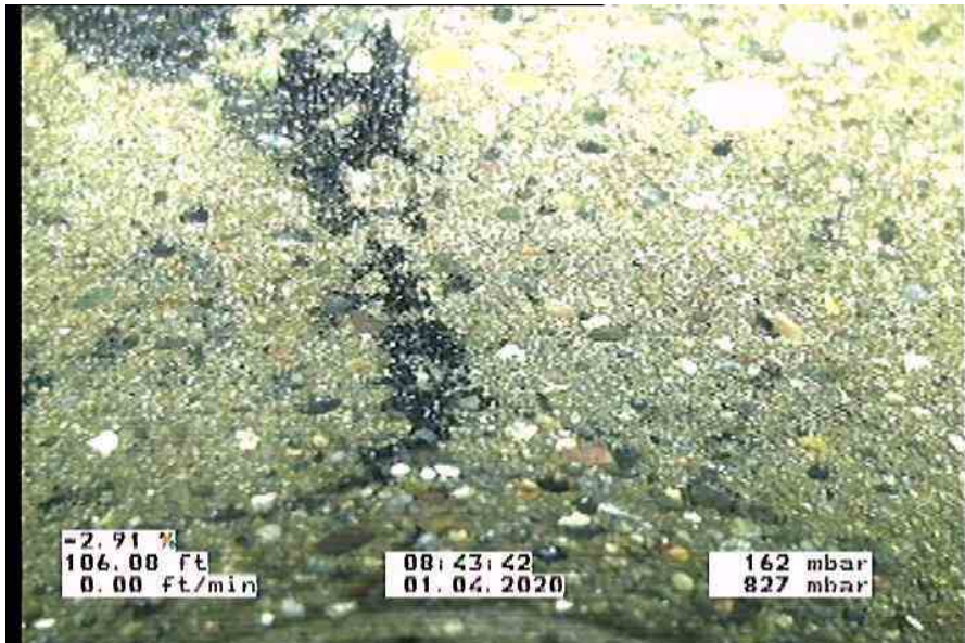
297_24bf6c94-8c3c-4a30-83bc-735eb4f0c968_20200401_084826_680.jpg, 00:07:17, 104.50ft Material Change, Concrete pipe (non reinforced)
